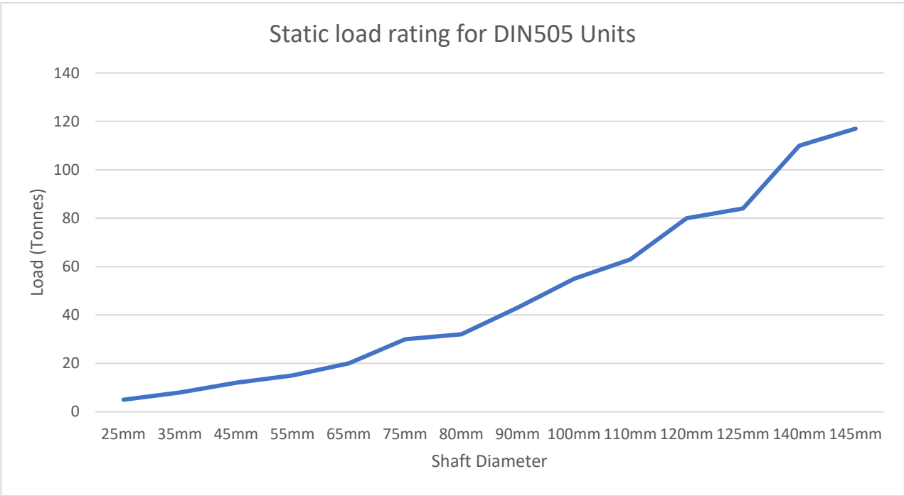
The chart shown above details the static load capacity of DIN505 units.
